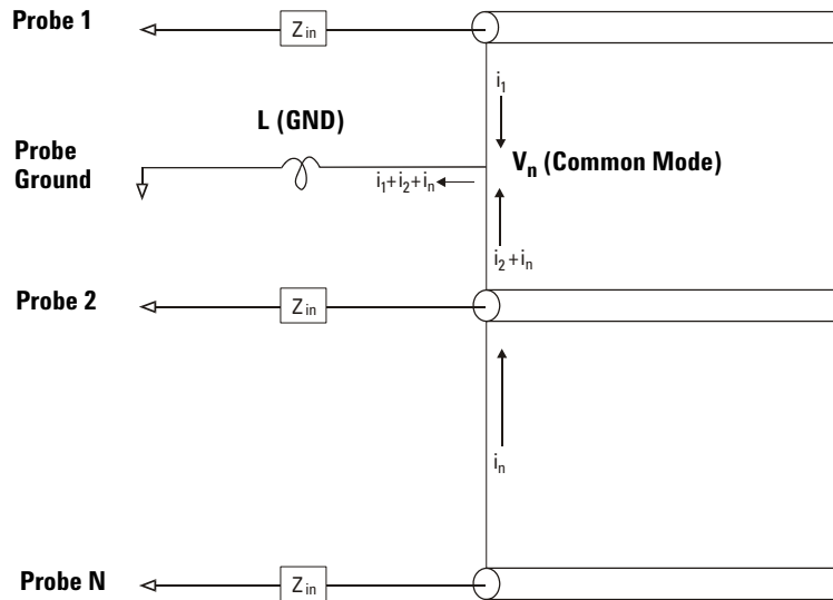
Figure 46 Common Mode Input Voltage Model
