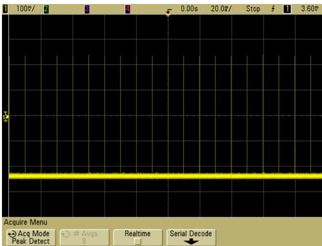
Figure 42 15 ns Narrow Pulse, 20 ns/div, Peak Detect Mode
