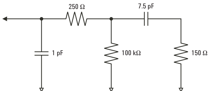
Figure 44 High-Frequency Probe Equivalent Circuit
